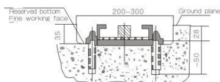
Sectional drawing of buried track group
