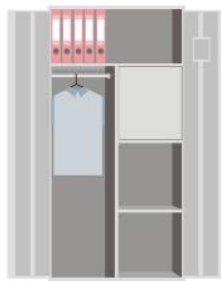
MY-OC-08 H1850*W900*D450mm
