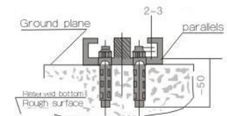
Ground track group section
