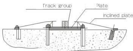
Sectional drawing of inclined plate ground track group
